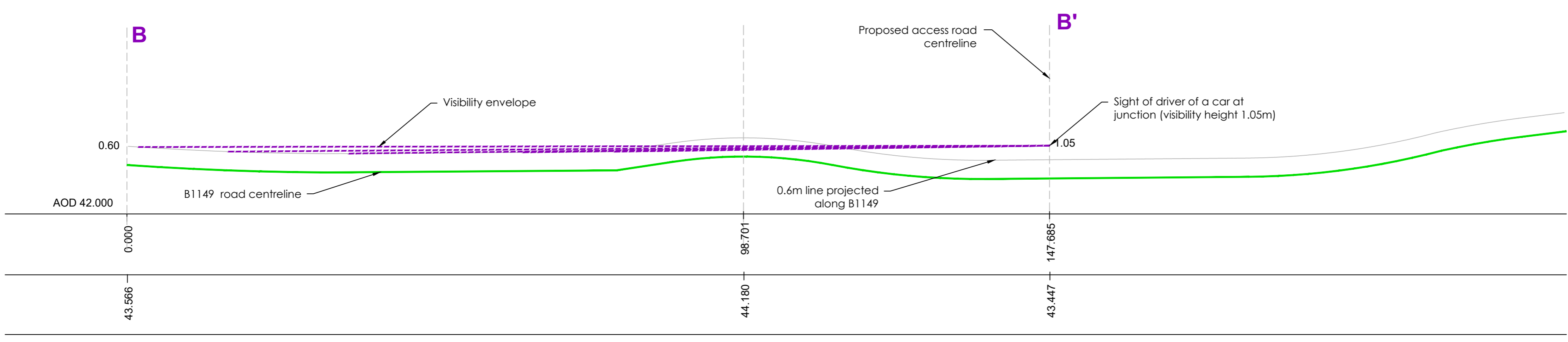
SECTION B-B' EXISTING LEVELS ALONG THE B1149 TO THE NORTH OF THE ACCESS ROAD (SCALE H:1:500 V:1:100)
